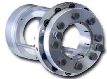
Clamping Systems for torque motors for the frictional connection of torque motors to machine shafts
