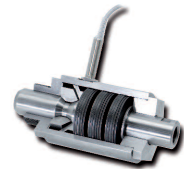
Force Limiters as overload protection in rods
