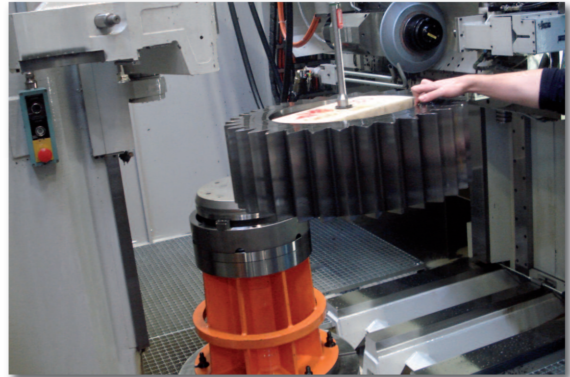
Grinding
