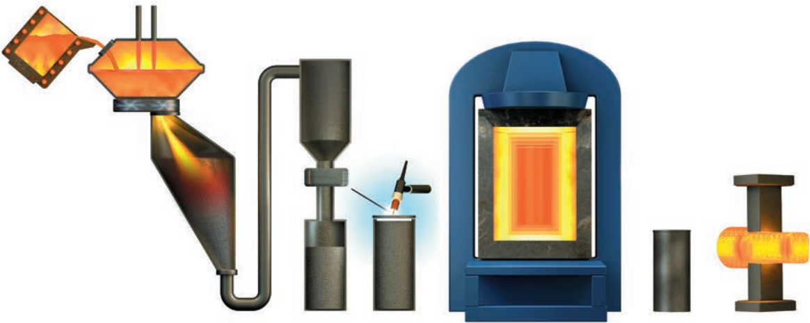
Figure 6. Schematic representation of the powder metallurgy (PM) route for producing tool steel.
