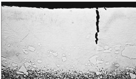
Photo 4. Surface of Uddeholm Sverker 21 after rough spark EDM. The white layer is brittle and contains cracks.
