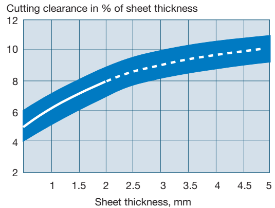
Figure 23. Recommended cutting clearance when shearing
