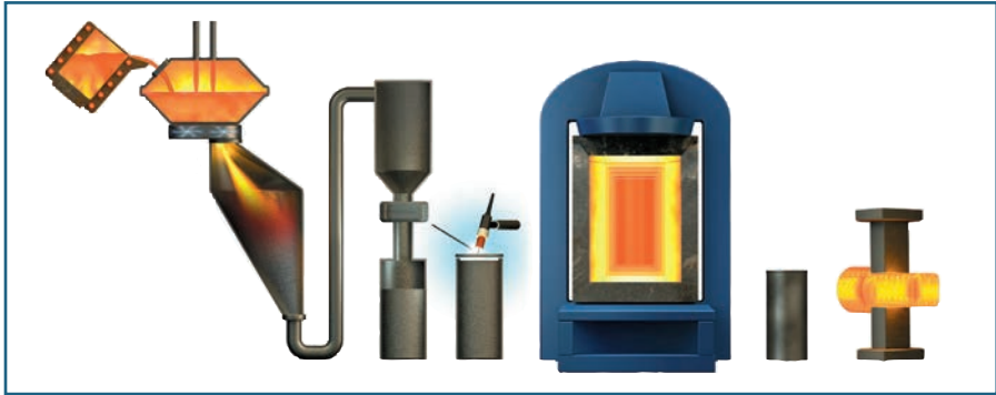
Figure 2. Powder metallurgy (PM) process.
