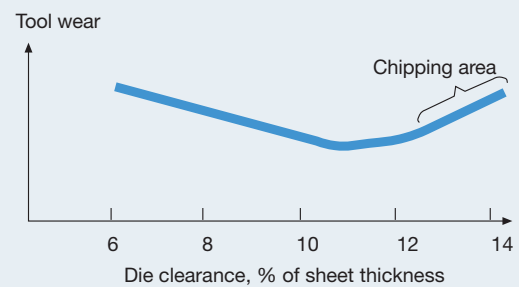
Figure 14. Relation between tool wear and die clearance when blanking in CR 1400T-MS, sheet thickness 1 mm.
