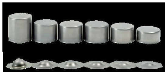
Figure 5. Maximum- cup height and dome height for deep drawing and stretch forming, respectively. Sheet steel grades (from left to right): CR4, CR600T-DP, CR800T- DP, CR1000T- DP, CR1200T- MS and CR1400T- MS.
