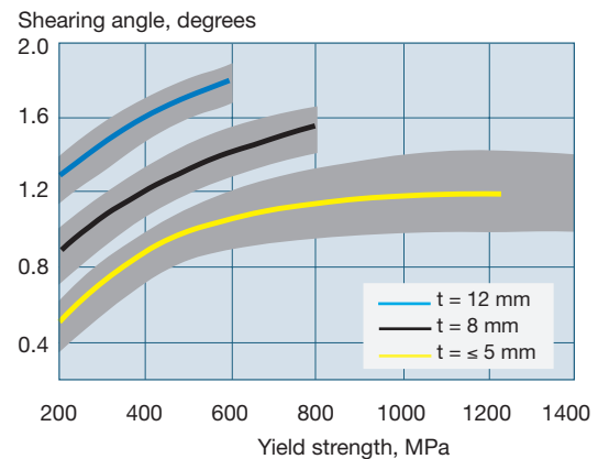
Figure 24. Recommended shearing angles depending on sheet thickness.
