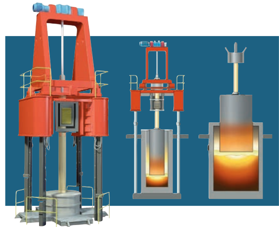
Figure 1. Electro slag remelting (ESR) process.
