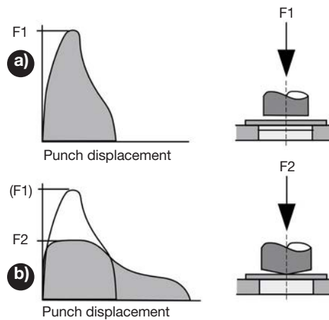
Figure 18. Blanking/punching force as a function of punch displacement for a) flat punch or b) chamfered punch.
