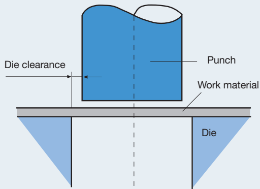
Figure 10. Die clearance definition.
