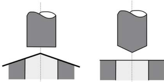
Figure 17. Chamfered tools for blanking and punching.
