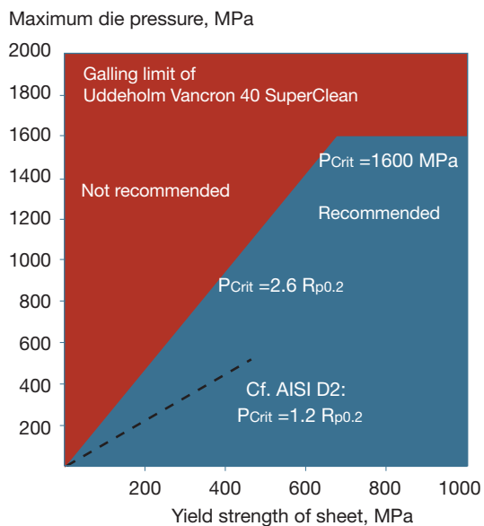
Figure 8. Limits to guide the use of uncoated Uddeholm Vancron 40 SuperClean to form carbon steel. Recommendations are based on application tests and FEM simulation. For comparison the approximate level of the galling limit of uncoated AISI D2 tool steel is included.
