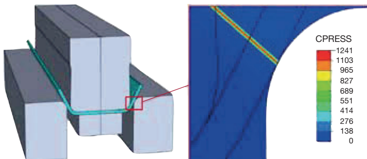
Figure 7. Computed die pressure distribution (MPa) from FE simulation of a U-bending application with CR 800T-DP.
