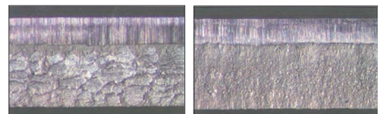
Figure 26. Sheet edge appearance for HR 700Y-MC, t = 2 mm with different cutting conditions. The left image indicates that cutting clearance and/or shearing angle is too large. The right image indicates that the cutting conditions are OK.
