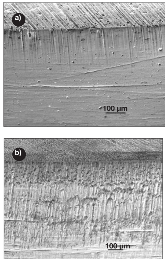
Figure 30. A blanking edge coated with a) PVD-coating (TiAlN) without galling and b) uncoated with galling after 200 000 parts produced in CR 800T-DP.
