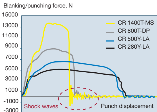
Figure 15. Blanking force and shock waves when punching advanced high strength steel grades.
