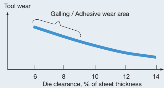
Figure 13. Relation between tool wear and die clearance when blanking in CR 800T-DP, sheet thickness = 1 mm.
