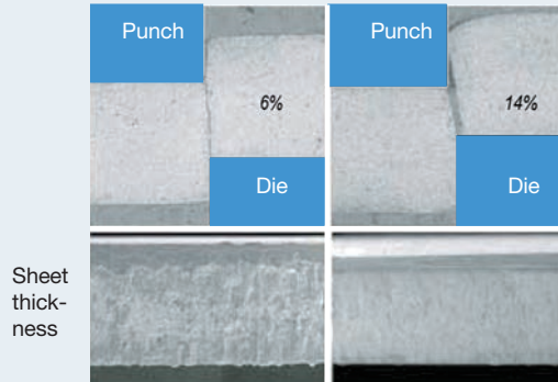
Figure 12. Edge cut with varying die clearance.
