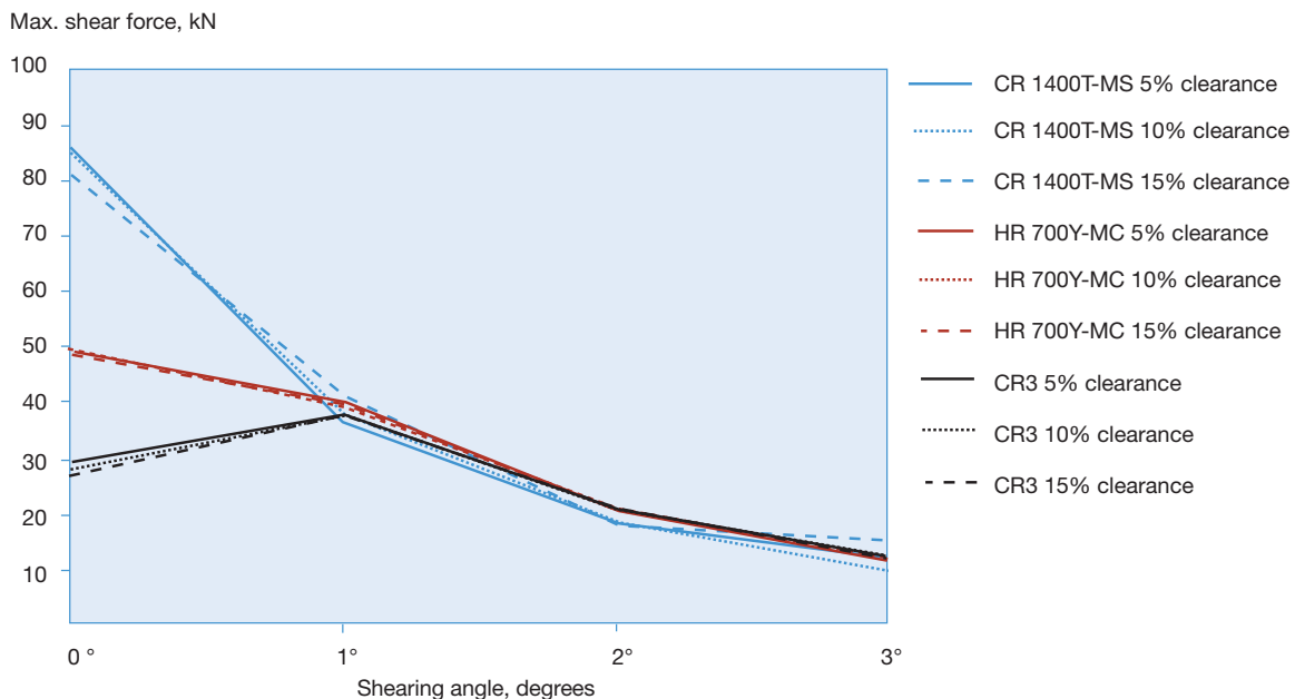
Figure 28. Shear force as a function of shearing angle for different cutting clearances. t = 2 mm.
