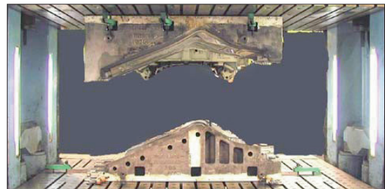
Figure 6. Complex stamping tool.
