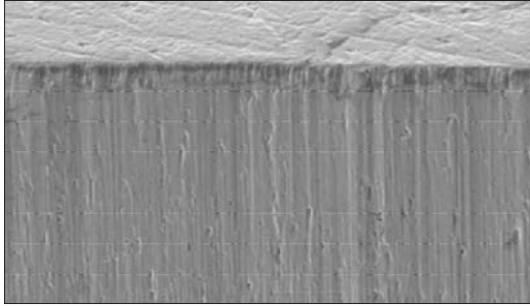
Figure 31. Typical tool wear of an uncoated blanking edge after 100 000 parts produced in CR 1400T-MS.
