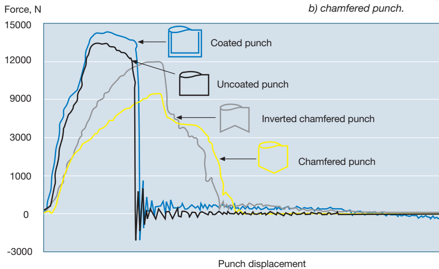
Figure 18. Blanking/punching force as a function of punch displacement for a) flat punch or b) chamfered punch.
