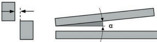
Figure 22. Cutting clearance and shearing angle respectively.
