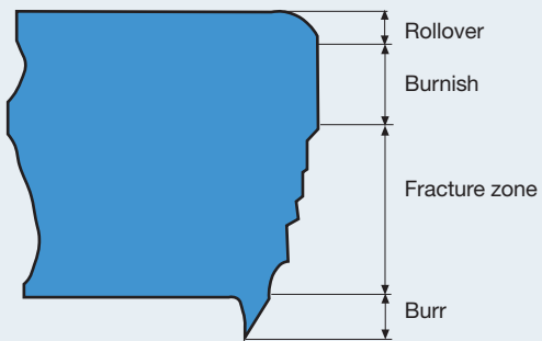
Figure 9. Appearance of a cut edge.
