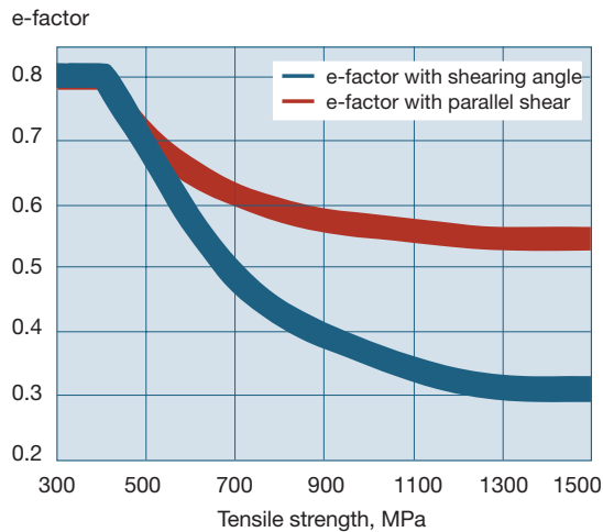
Figure 29. e-factor as a function of the work material tensile strength.
