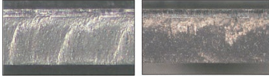
Figure 27. Sheet edge appearance for CR 1400T-MS, t = 2 mm with different cutting conditions. The left image indicates that cutting clearance and/or shearing angle is too large. The right image indicates that the cutting conditions are OK.
