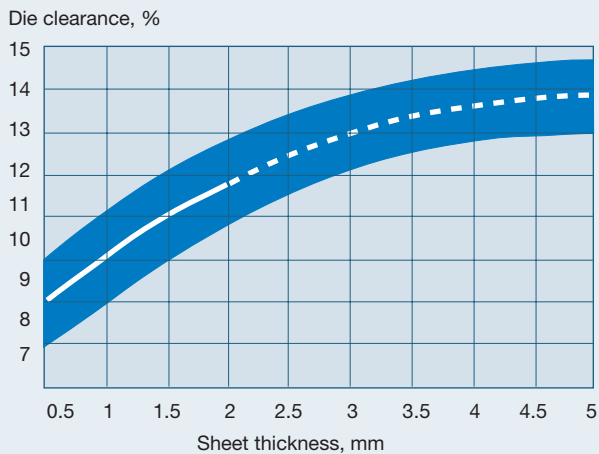
Figure 11. Recommended die clearance for blanking/punching advanced high strength steel.
