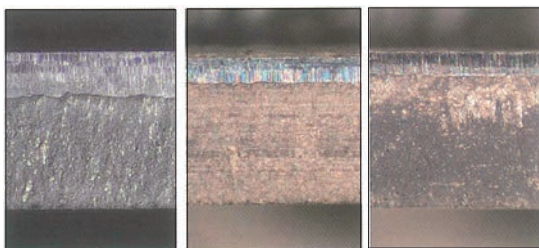
Figure 25. Sheet edge appearance for HR 700Y-MC, CR 800T-DP and CR 1400T-MS respectively in thickness 2 mm with 7% cutting clearance and 1° shearing angle.
