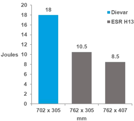
Figure 6 clearly shows Uddeholm Dievar is tougher at higher hardness to premium H13
