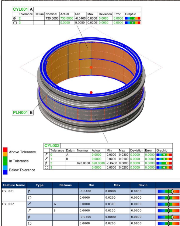
TOP: Bearing outer race inspection in progress by touch probing and scanning in a single 10-minute cycle BOTTOM: A typical quality report automatically generated in LK CAMIO 2021 after inspection of a Timken bearing
